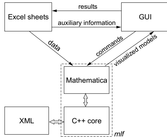
Figure 3: The architecture of PaperMiner which, is based on mif .
